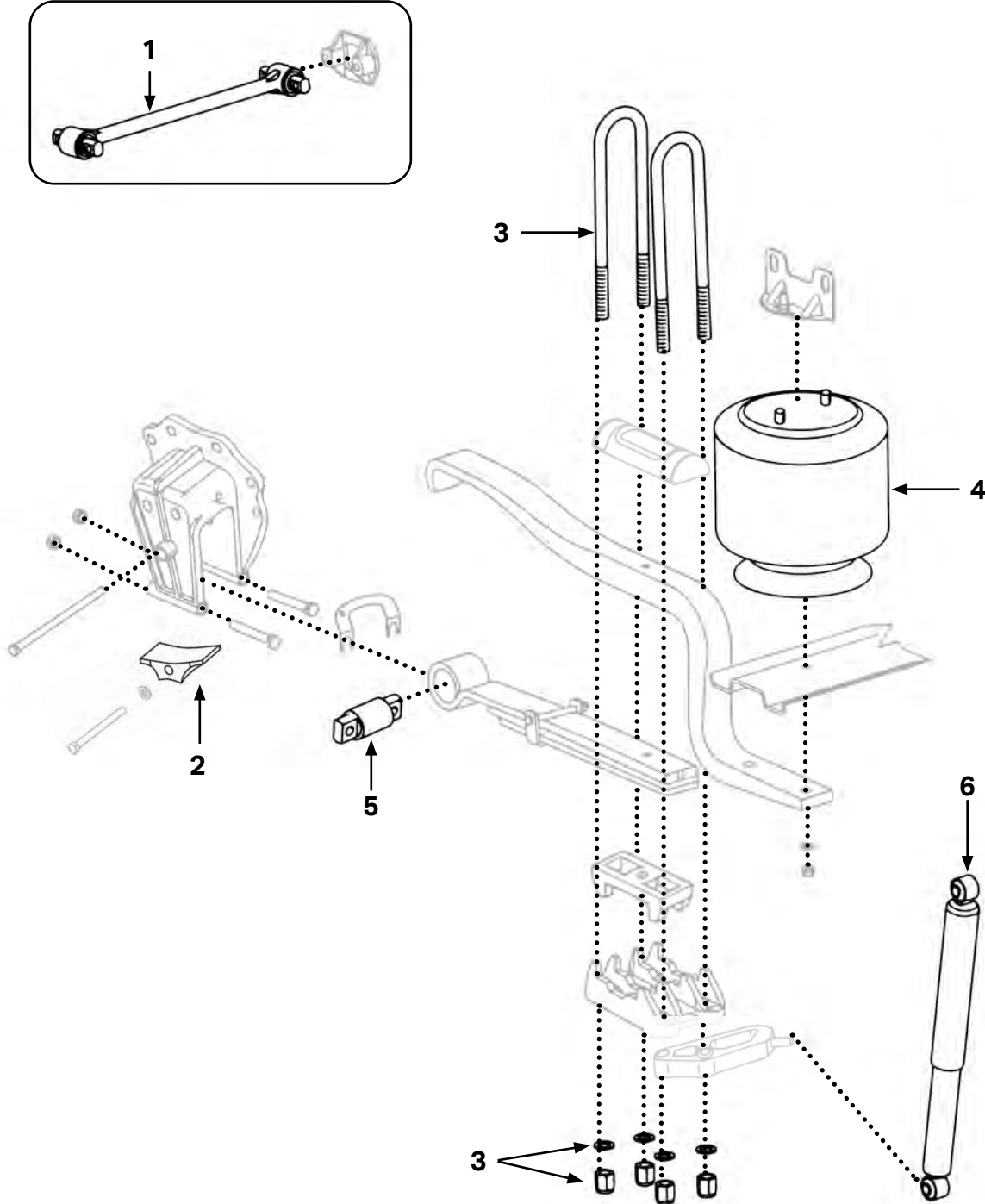
STRADDLE PIN STYLE TRANSVERSE ROD
