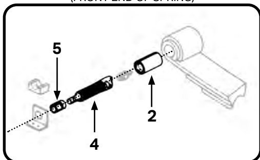
THREADED PINS & BUSHINGS (FRONT END OF SPRING)
