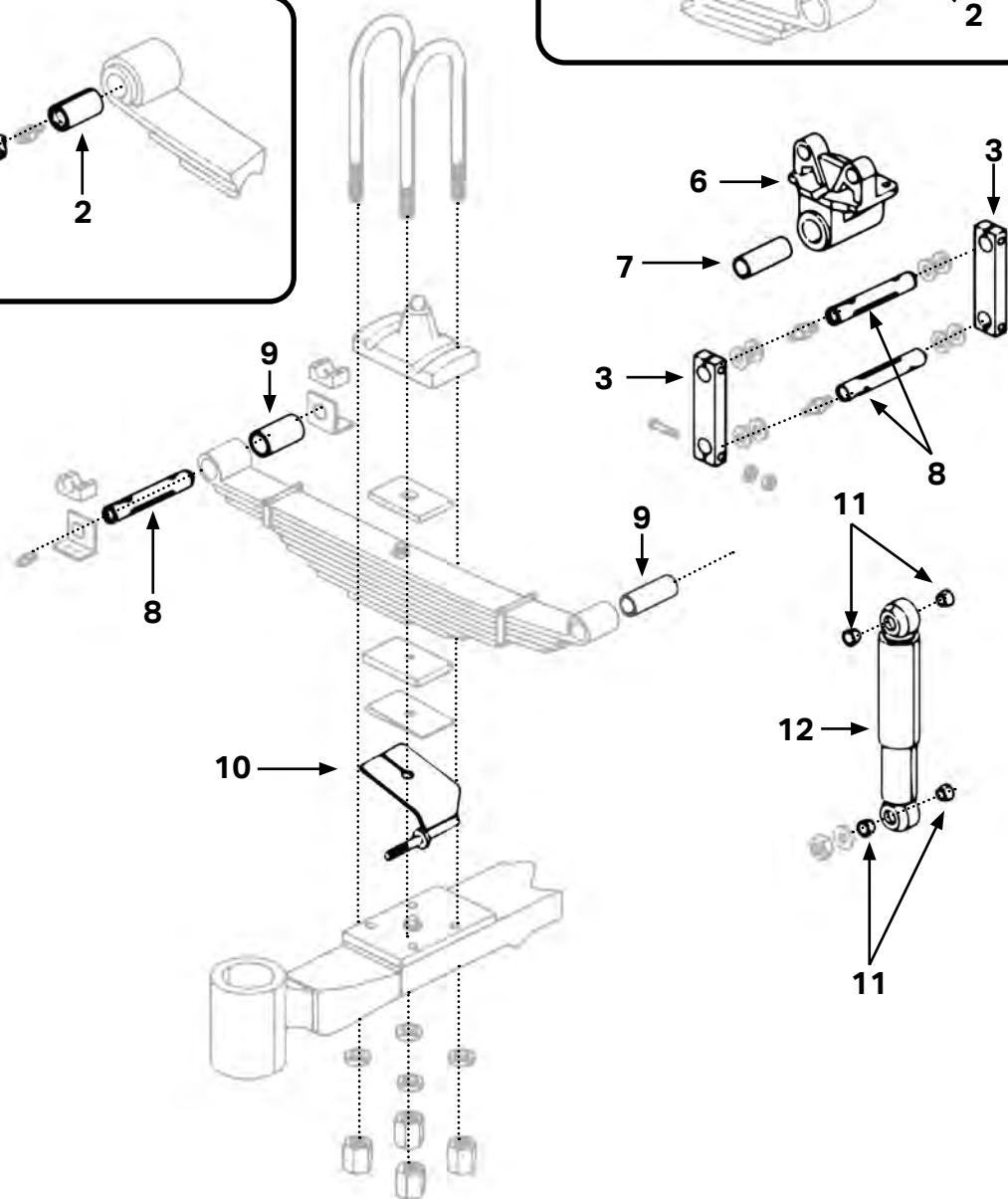
THREADED PINS & BUSHINGS (FRONT END OF SPRING)
