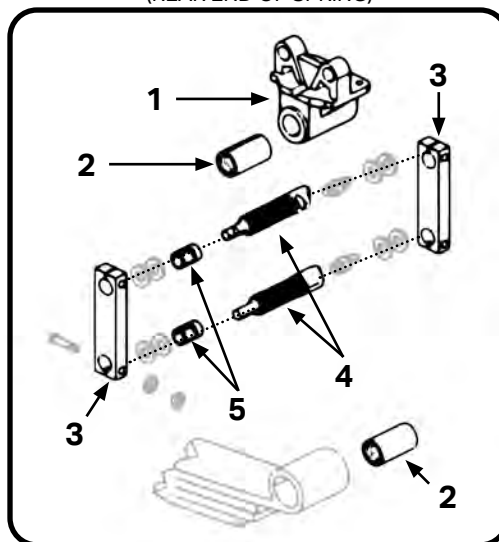
THREADED PINS & BUSHINGS (REAR END OF SPRING)
